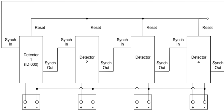
Series Synch Connections
