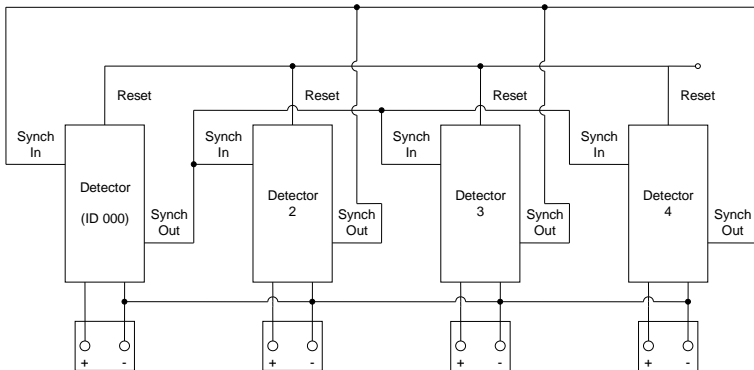
Parallel Synch Connections
