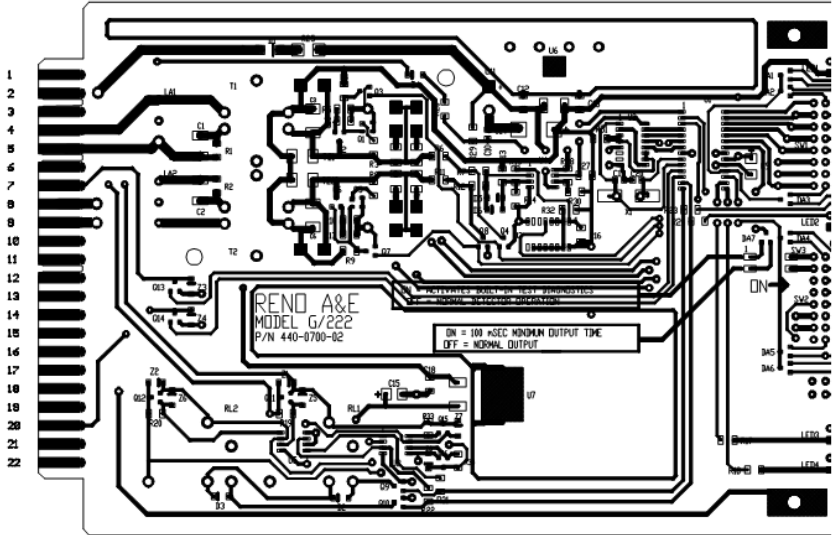
Parts Locator
