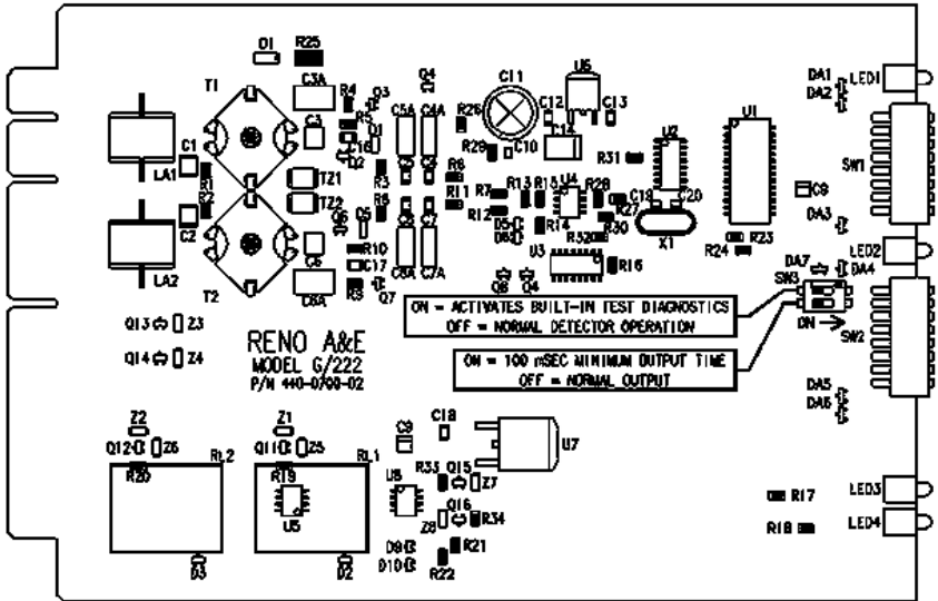
Parts Locator
