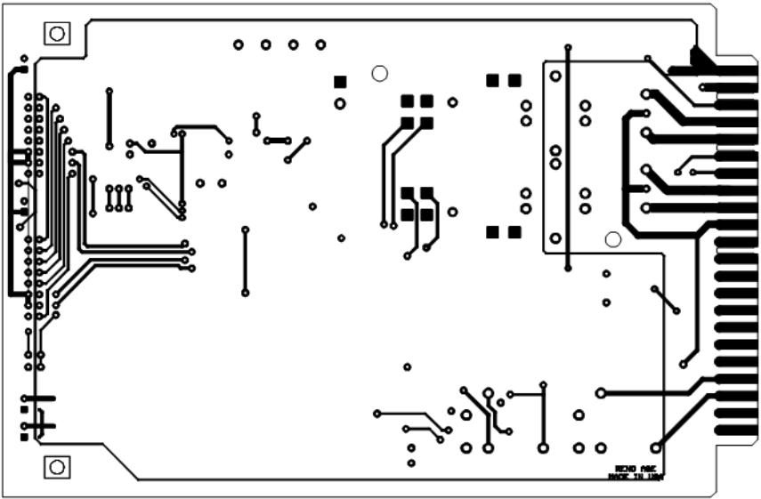
Bottom View
