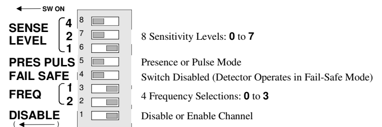
Front Panel Eight-position DIP Switch (Factory Default Settings Shown)
